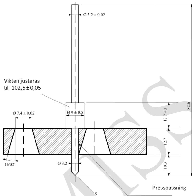
Figur 1: Penetrometer
